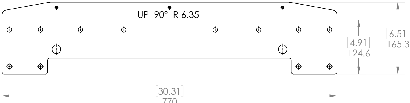
FLAT PATTERN
